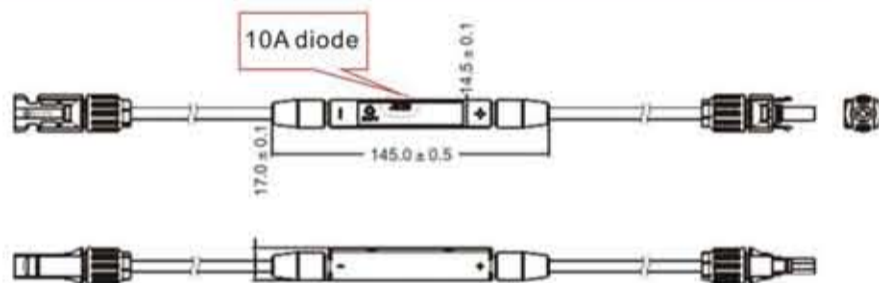
Standard IP67 waterproof junction box with 90CM cable and MC4 Connectors.
